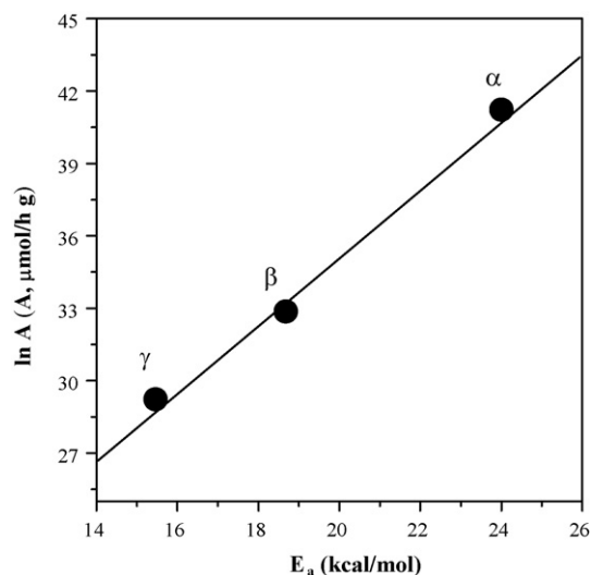
Fig. 10. Compensation effect in ionone isomer formation on HPAS.
