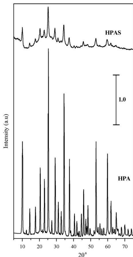
Fig. 1. XRD patterns of HPA and HPAS samples.
